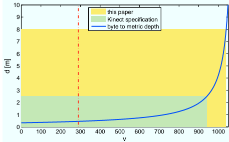
Fig. 2. Kinect depth characteristics. The blue line is the function that relates the byte values of the range image to metric depth, the red line is the sensor’s minimal measurable depth. The dark green area indicates the adequate play space recommended in the Kinect User Manual, the yellow area is the range considered in this paper for detecting people. Notice that we address the problem of people detection at nearly 4\times the suggested working range, where depth resolution is becoming increasingly coarser.
